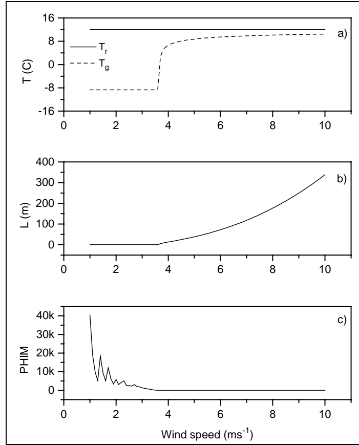
Figure 8. A plot at t = 0.125 hr of a) the estimated surface temperature ( T_g ), b) the estimated M-O scaling length ( L ), and c) the estimated dimensionless wind shear ( \phi_m ) as a function of the 5-m reference height wind speed ( U_r ).
