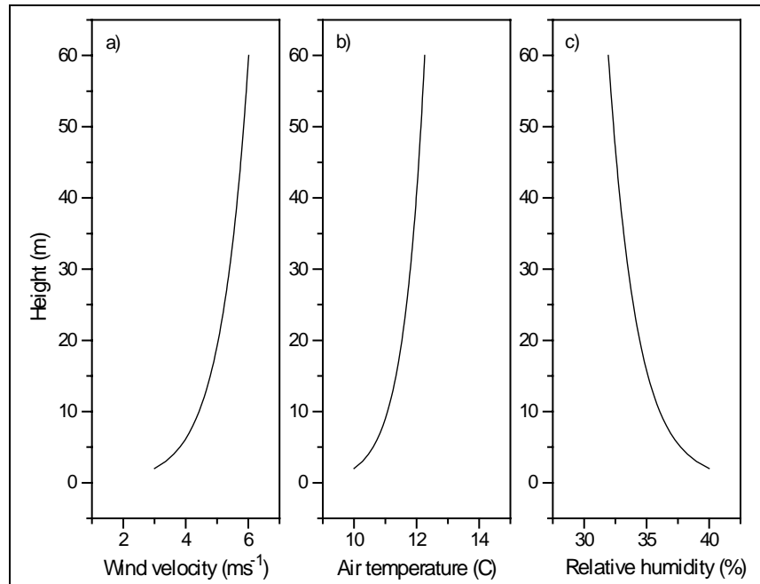
Figure 2. Typical similarity-based profiles for the nighttime case derived from the energy budget model: a) wind velocity (in units \text{ms}^{-1} ), b) air temperature (in units C), and c) relative humidity (in percent).
